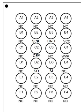
TFBGA-24 (Package: JG)
