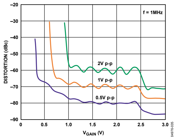
Figure 34. HD3 vs. V_{\text{GAIN}} at Three Output Voltages, High Gain (See Figure 53)
