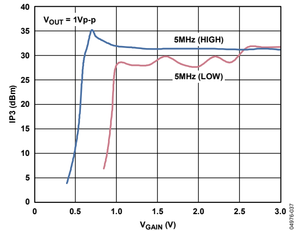
Figure 36. Output Referred IP3 (OIP3) vs. V_{\text{GAIN}}
