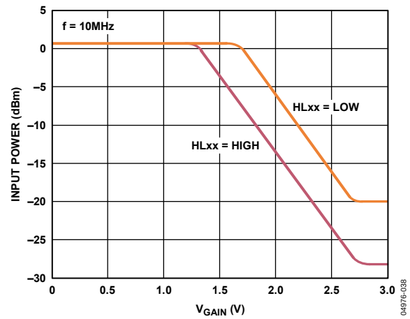
Figure 37. Input P1dB (IP1dB) vs. V_{\text{GAIN}}
