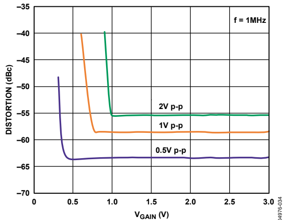
Figure 33. HD2 vs. V_{\text{GAIN}} at Three Output Voltages, High Gain, f = 1 \text{ MHz} (See Figure 53)
