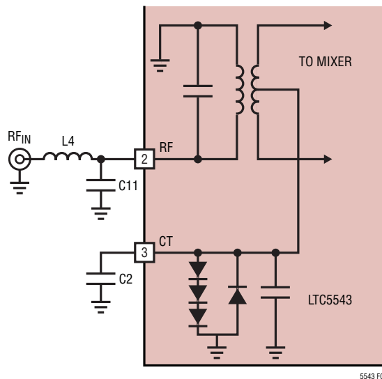
Figure 3. RF Input Schematic
