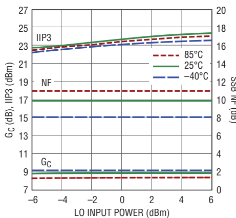
2300MHz Conversion Gain, IIP3 and NF vs LO Power
