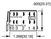
VC1 CONNECTOR HOUSING
