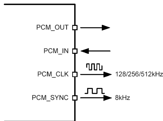
Figure 13: PCM Interface Master
