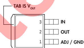
DD PACKAGE (D 2 Pak) (Top View)
