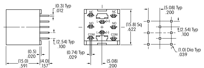
AT712 Double Pole • Straight PC Terminals
