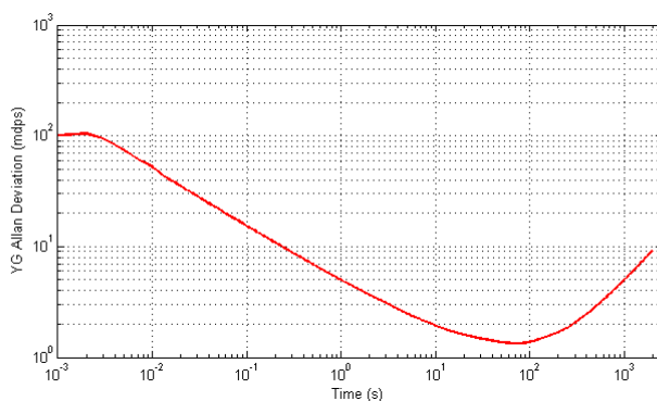
Y-Axis Gyroscope – Example Allan Variance Plot
