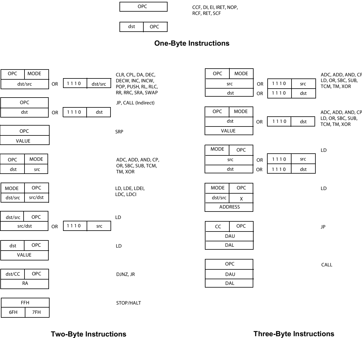
Figure 47. Instruction Formats
