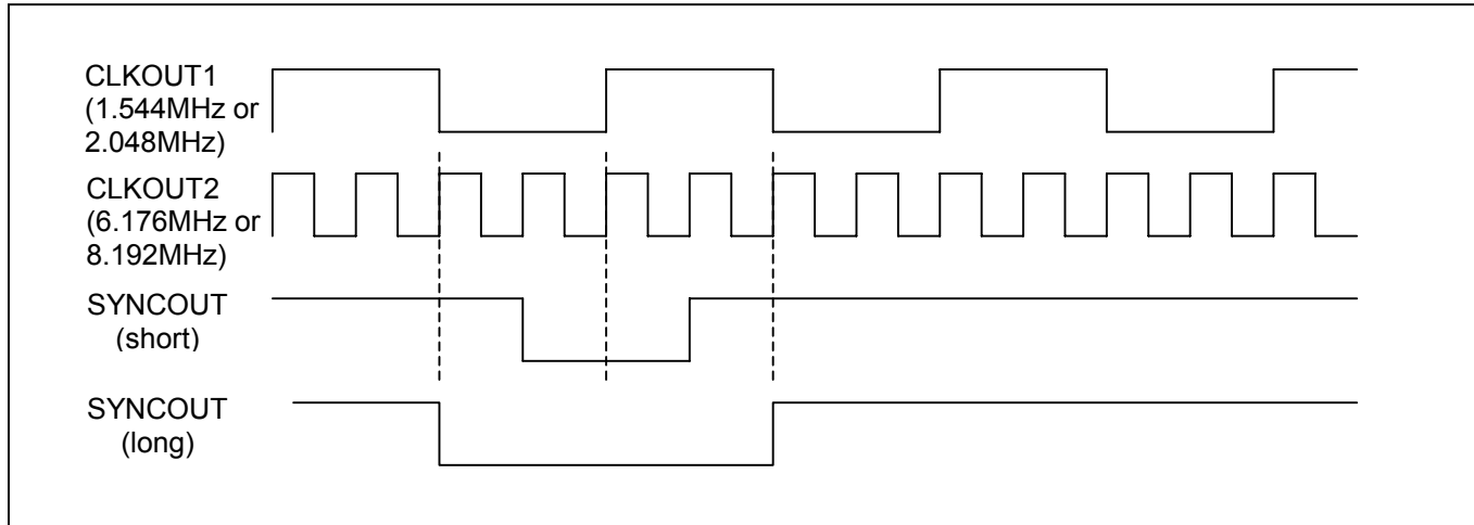
Figure 4-4. Output Frame-Sync Alignment When \text{CLKOUT2} = 4 \times \text{CLKOUT1}
