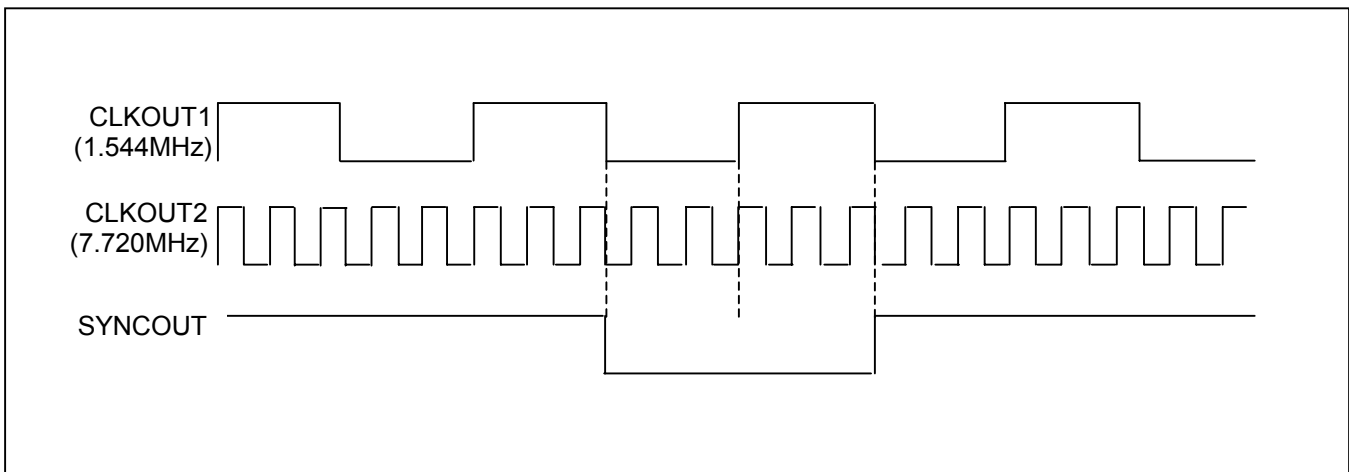
Figure 4-5. Output Frame-Sync Alignment When \text{CLKOUT2} = 5 \times \text{CLKOUT1}
