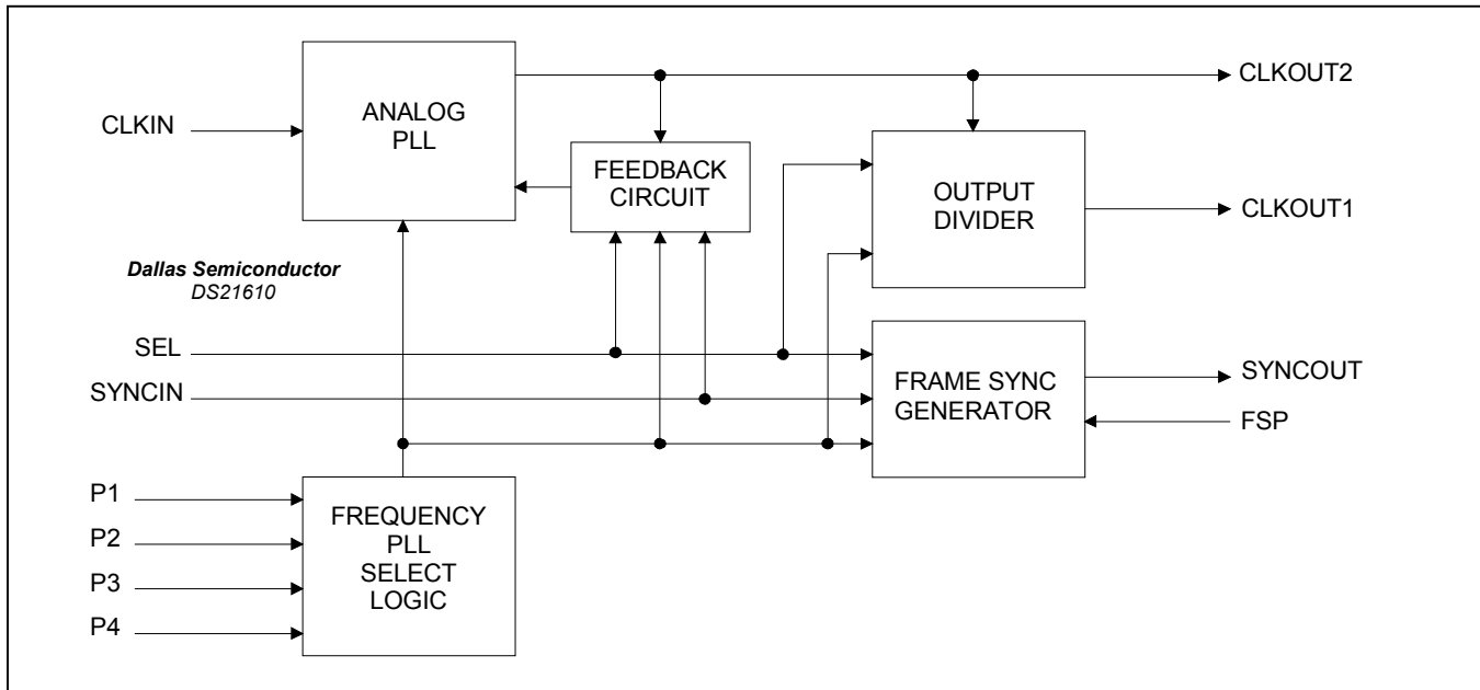
Figure 1-1. Block Diagram
