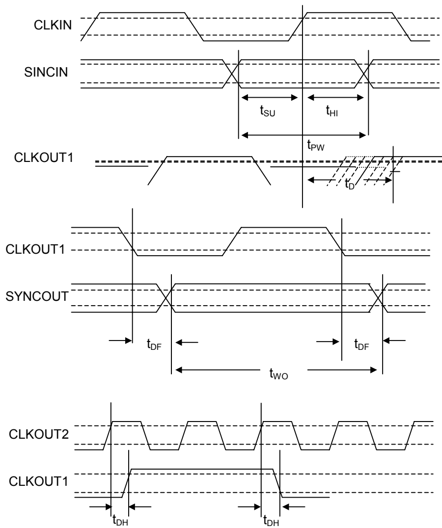
Figure 4-1. SYNCIN/CLKIN to CLKOUT1/SYNCOUT and CLKOUT2
