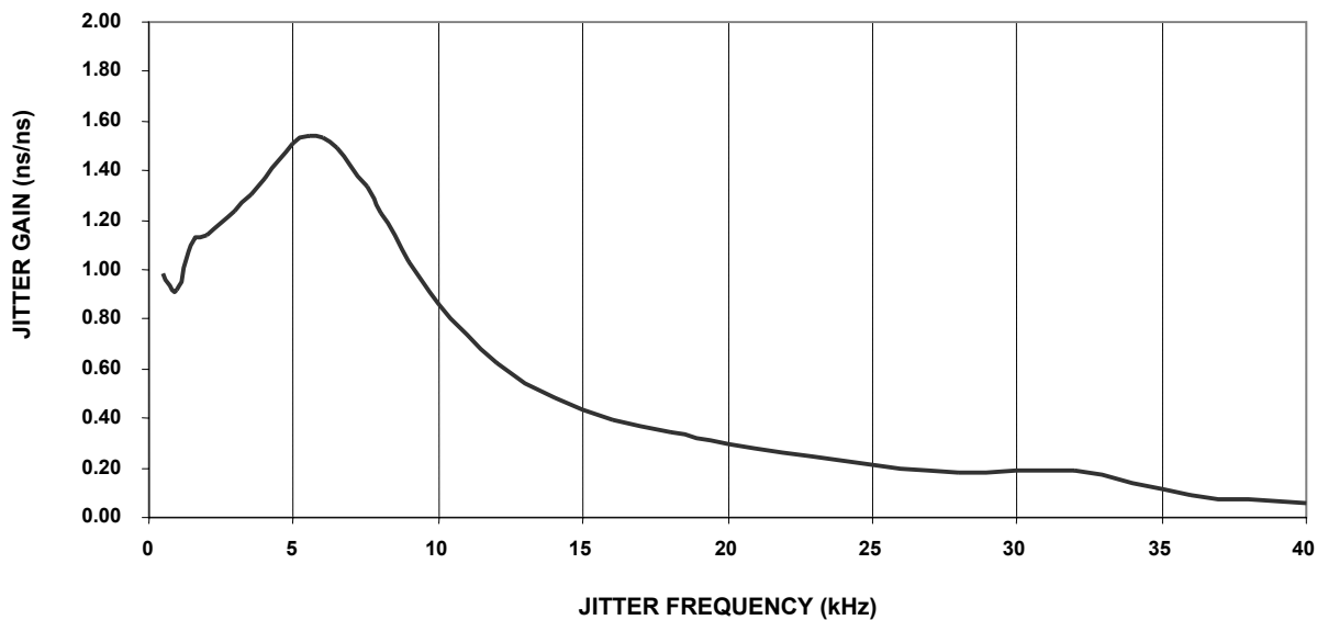
Figure 3-1. Nominal Jitter Transfer (1.544MHz CLKIN to 2.048MHz CLKOUT1)
