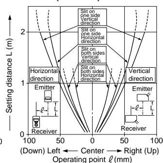
Parallel deviation with rectangular slit masks ( 1 \times 6\text{mm} )
