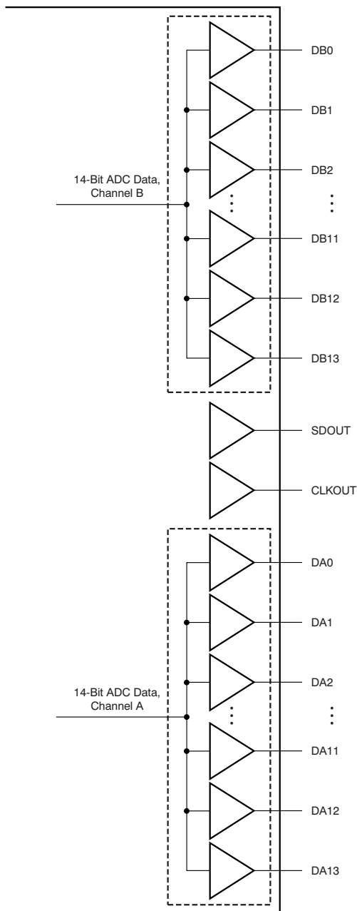
Figure 170. CMOS Outputs
