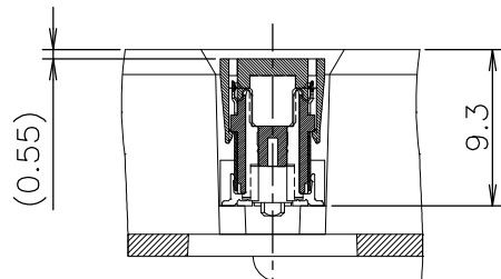
SECT. D-D (SCALE 2:1)
