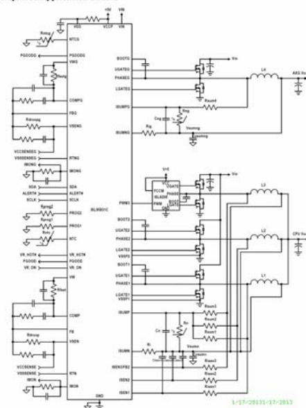
Simplified Application Circuit
