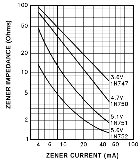
FIGURE 2 ZENER IMPEDANCE VS ZENER CURRENT (TYPICAL)
