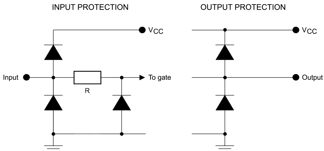
Figure 1. Input and output equivalent circuit diagram
