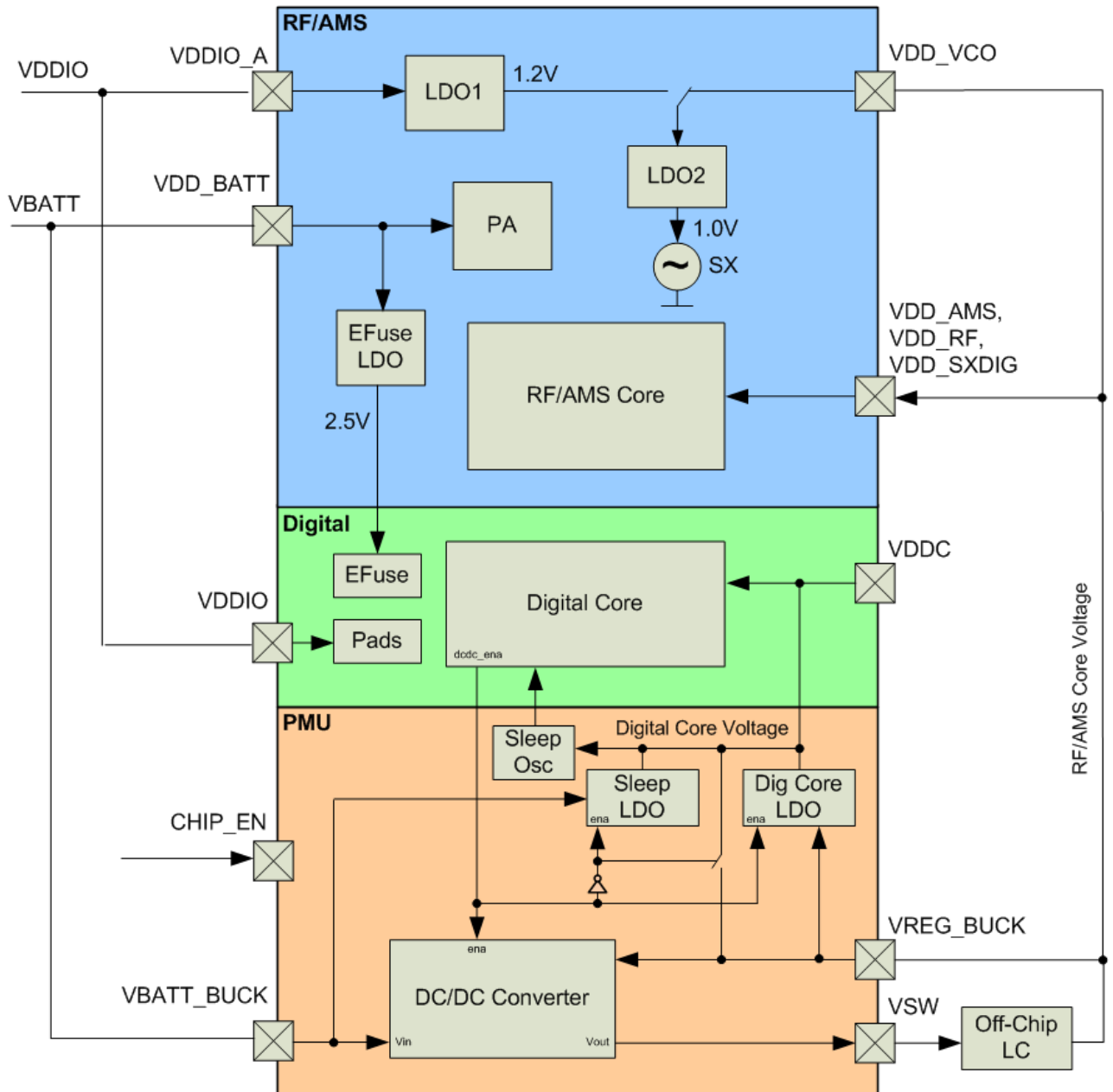
Figure 9-1. Power Architecture
