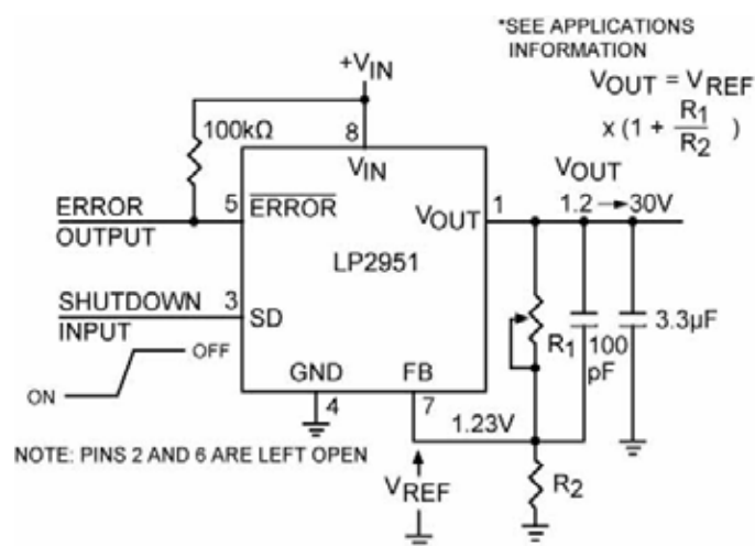
Figure 2. Adjustable Regulator
