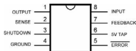
DIP (N) and SOIC (M)
