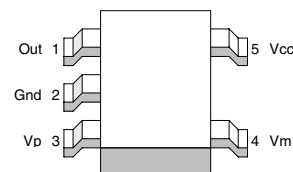
Pin connections (top view)
