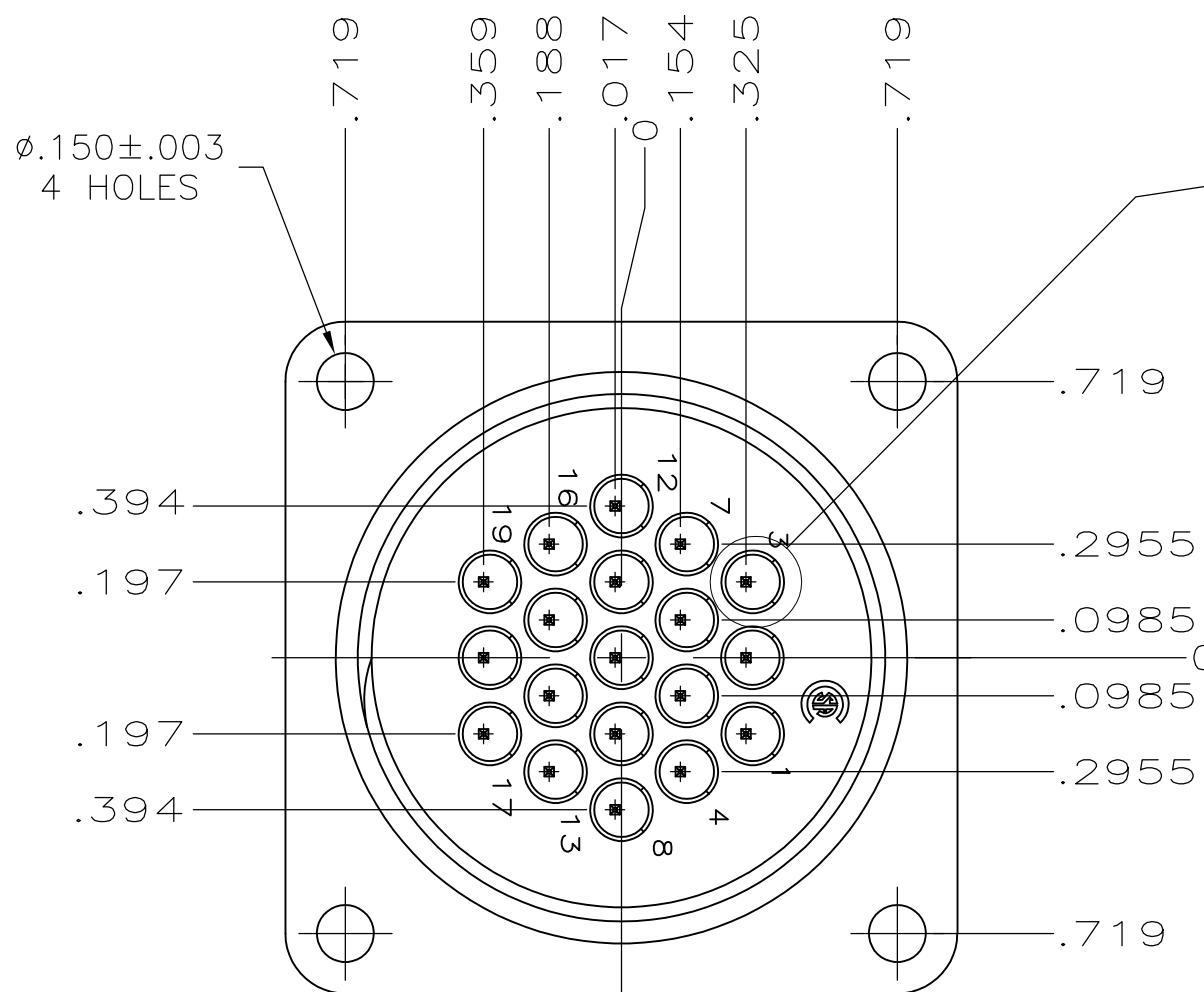
VIEW B-B
