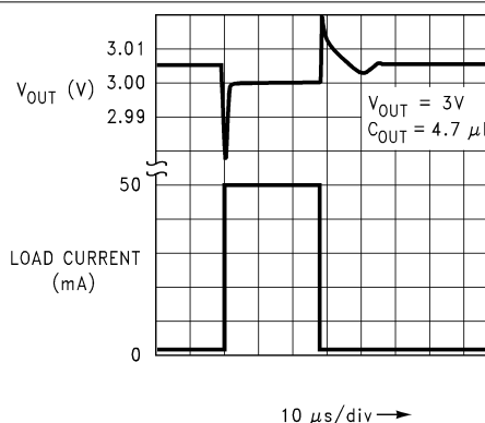
Figure 7-10. Load Transient Response (Legacy chip)
