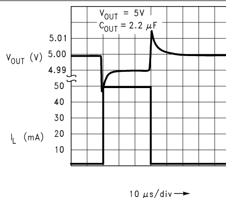
Figure 7-12. Load Transient Response (Legacy chip)
