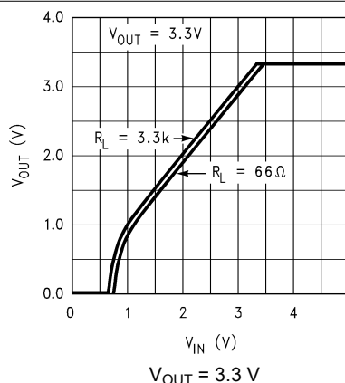
Figure 5-6. Output Voltage vs V_{IN} (Legacy Chip)
