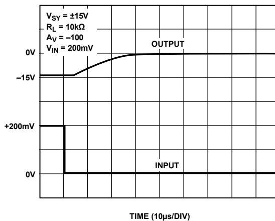
Figure 18. Positive Overvoltage Recovery
