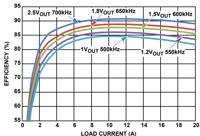
FIGURE 5. EFFICIENCY vs LOAD CURRENT (12V IN )
