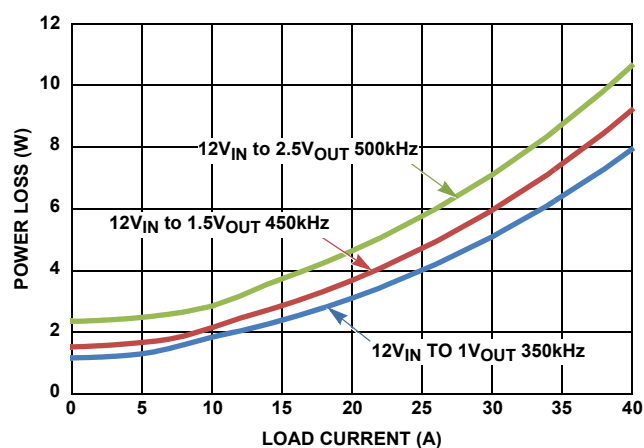
FIGURE 37. POWER LOSS CURVES OF 12V IN
