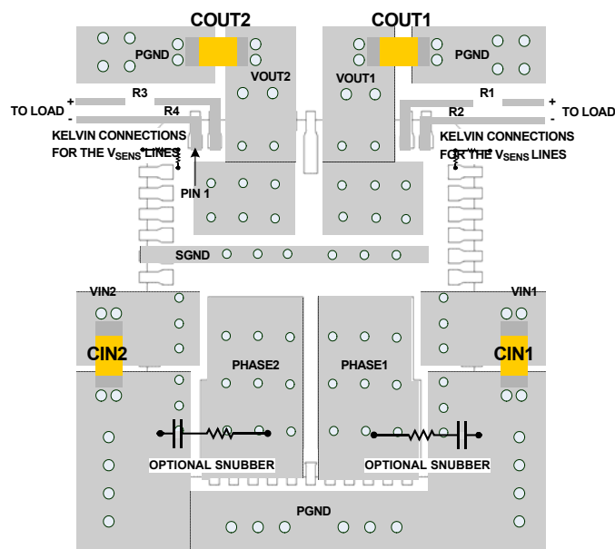
FIGURE 35. RECOMMENDED LAYOUT
