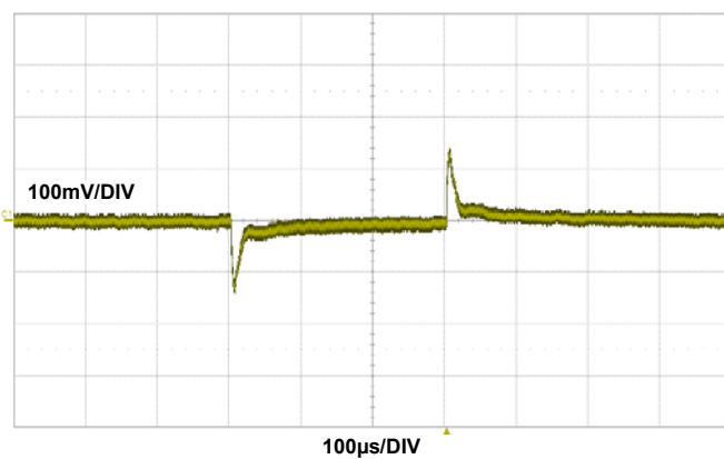
FIGURE 16. 1.5V OUT DUAL PHASE SINGLE OUTPUT TRANSIENT RESPONSE, I_{OUT} = 0A TO 20A , f_{SW} = 400kHz , C_{OUT} = 330\mu F POSCAP+ 10\mu F + 5 \times 100\mu F CERAMIC CAPACITOR
