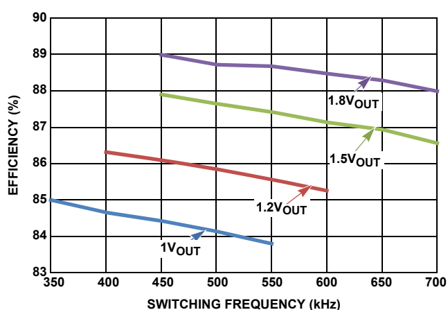
FIGURE 8. EFFICIENCY vs SWITCHING FREQUENCY AT V_{\text{IN}} = 5\text{V} (PARALLEL SINGLE OUTPUT, AS SHOWN IN Figure 24) AND I_{\text{OUT}} = 36\text{A} FOR VARIOUS OUTPUT VOLTAGES
