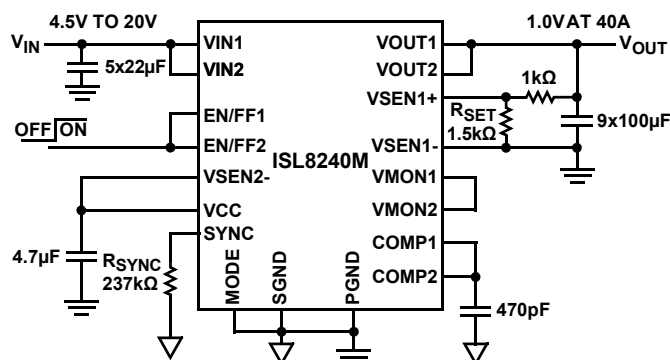
FIGURE 1. COMPLETE 40A STEP-DOWN POWER SUPPLY
