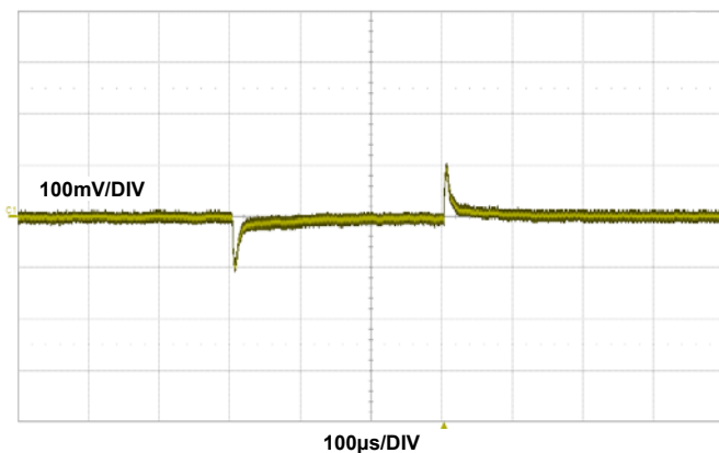
FIGURE 15. 1V OUT DUAL PHASE SINGLE OUTPUT TRANSIENT RESPONSE, I_{OUT} = 0A TO 20A , f_{SW} = 350kHz , C_{OUT} = 330\mu F POSCAP+ 10\mu F + 5 \times 100\mu F CERAMIC CAPACITOR
