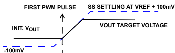
FIGURE 31. SOFT-START WITH V_{OUT} < \text{TARGET VOLTAGE}
