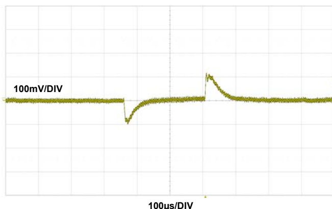
FIGURE 18. 1V OUT SIX PHASE SINGLE OUTPUT TRANSIENT RESPONSE, I_{OUT} = 0A TO 60A , f_{SW} = 350kHz , C_{OUT} = 6 \times 330\mu F POSCAP+ 7 \times 47\mu F + 6 \times 100\mu F CERAMIC CAPACITOR
