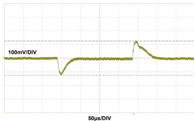
FIGURE 17. 0.9V OUT FOUR PHASE SINGLE OUTPUT TRANSIENT RESPONSE, I_{OUT} = 0A TO 40A , f_{SW} = 350kHz , C_{OUT} = 6 \times 330\mu F POSCAP+ 7 \times 47\mu F + 4 \times 100\mu F CERAMIC CAPACITOR
