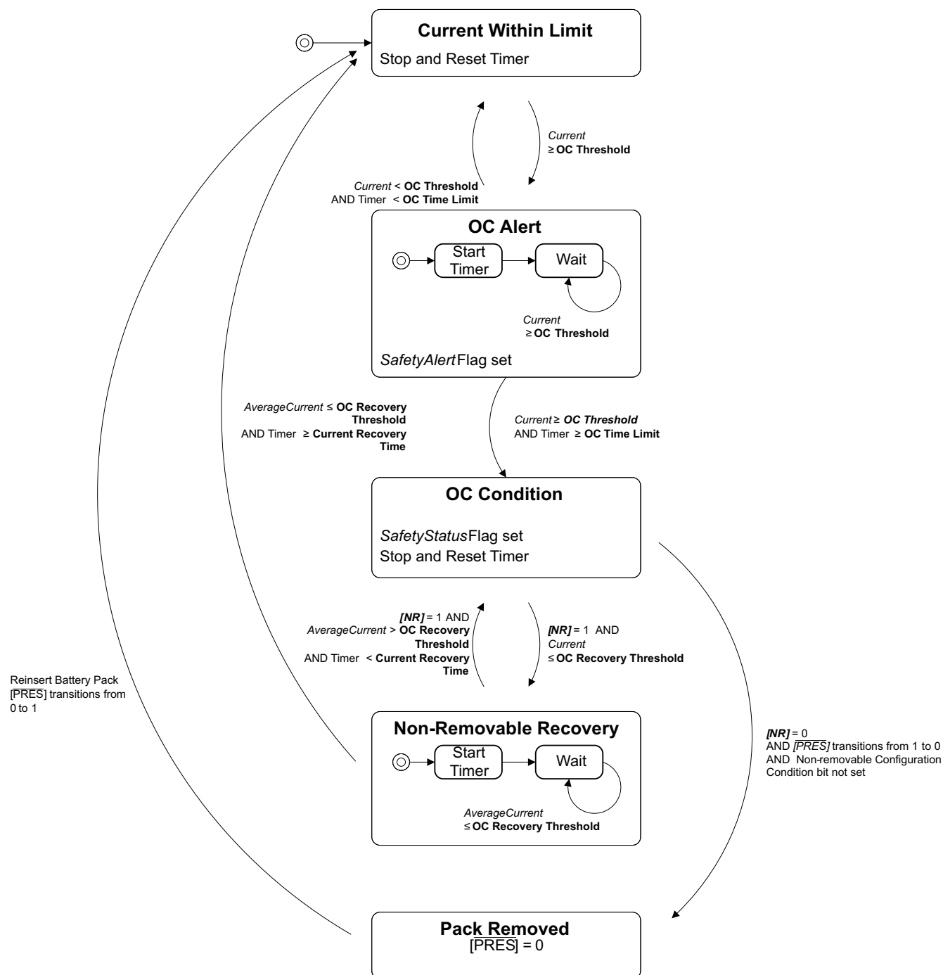
Figure 2-2. OC Protection
