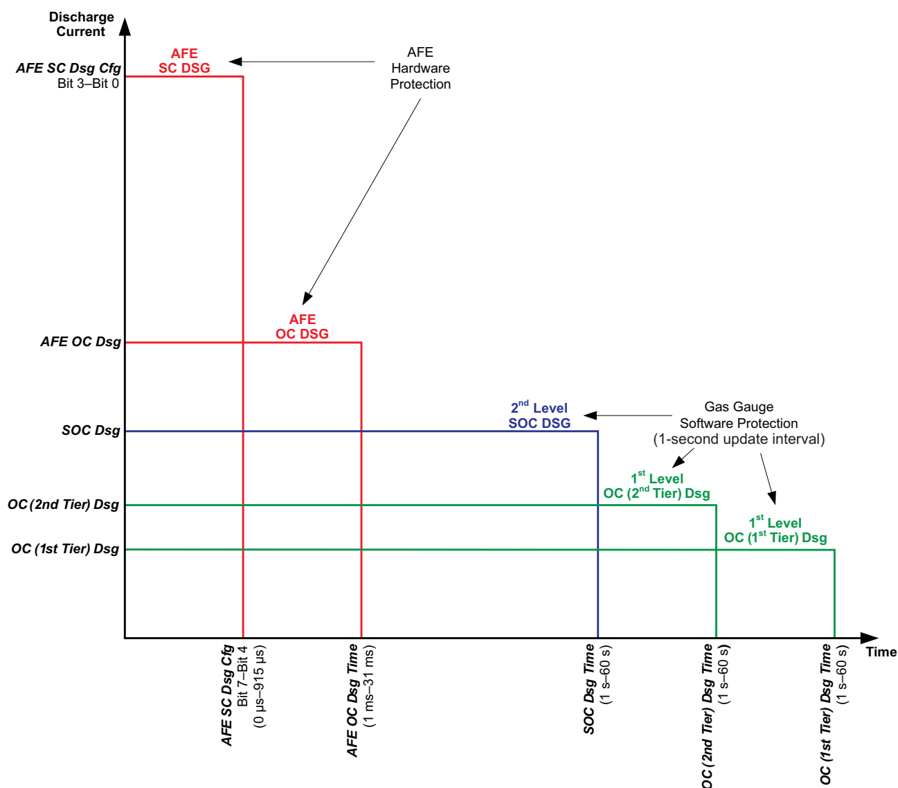
Figure 2-3. Overcurrent Protection Levels
