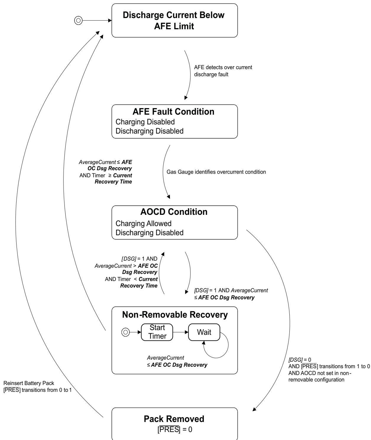
Figure 2-4. AFE Discharge Overcurrent Protection
