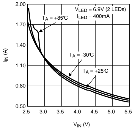
Figure 3. Input Current vs Input Voltage
