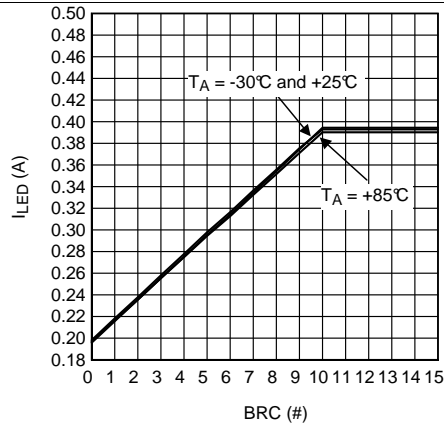
Figure 1. LED Current vs Brightness Code
