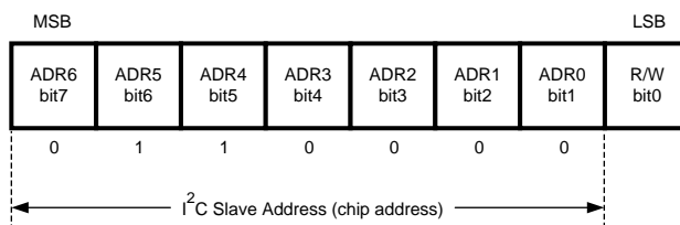
Figure 44. Device Address
