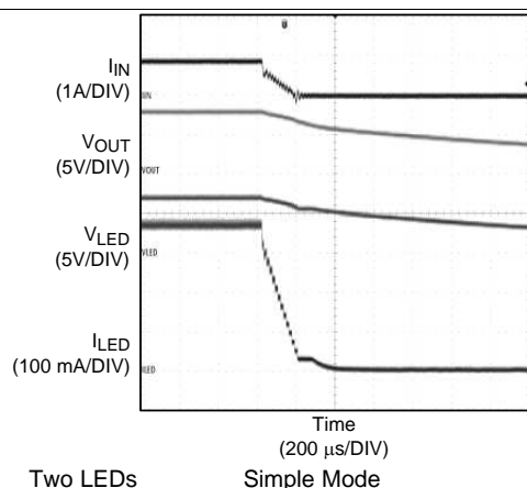
Figure 29. Ramp-Down
