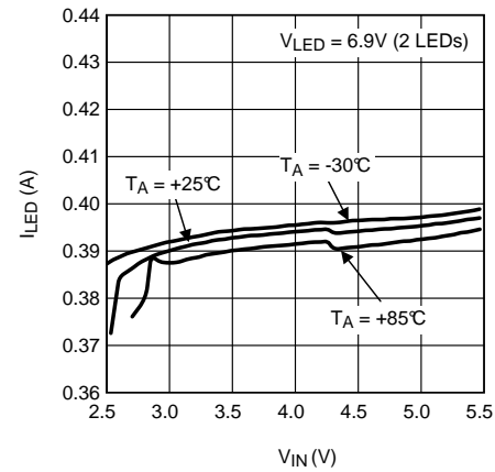
Figure 2. LED Current vs Input Voltage
