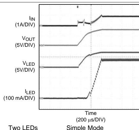
Figure 28. Start-Up
