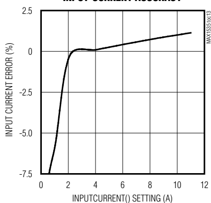
INPUT-CURRENT ACCURACY
