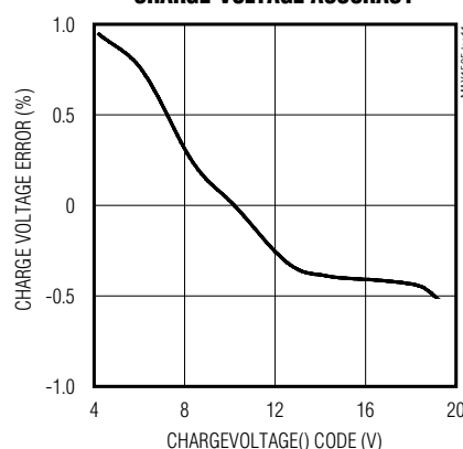
CHARGE-VOLTAGE ACCURACY
