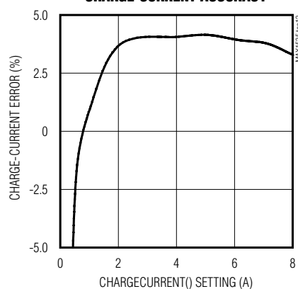
CHARGE-CURRENT ACCURACY
