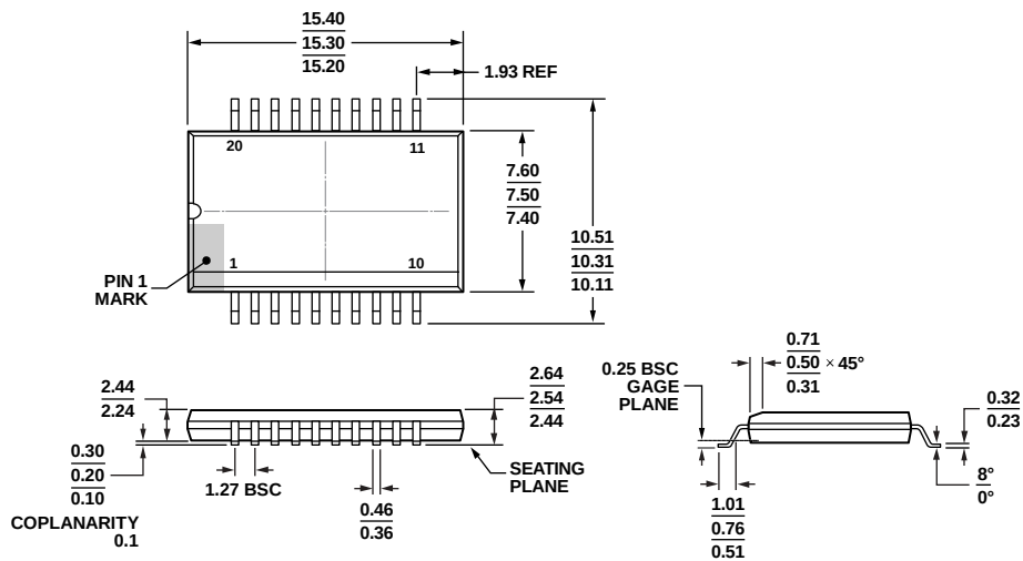
Figure 59. 20-Lead Standard Small Outline Package, with Increased Creepage [SOIC_IC] Wide Body (RI-20-1) Dimensions shown in millimeters
