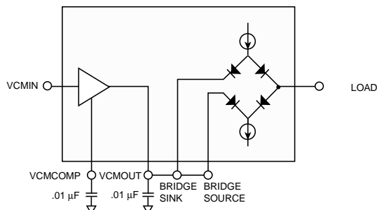
Figure 3. Commutating Voltage Compensation
