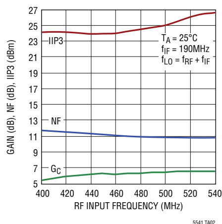
Gain, NF and IIP3 vs RF Frequency
