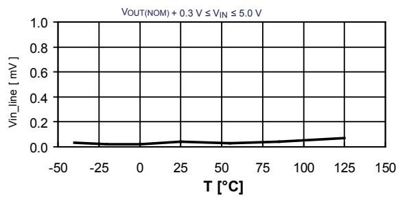
Figure 10. V_{in\_line} vs. temp. ( V_{OUT(NOM)} + 0.3 V \leq V_{IN} \leq 5.0 V )
