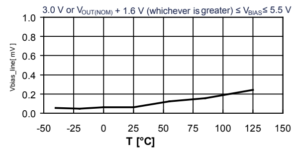
Figure 11. V_{bias\_line} vs. temp. ( 3.0 V or V_{OUT(NOM)} + 1.6 V , whichever is greater, \leq V_{BIAS} \leq 5.5 V )
