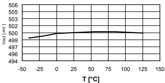
Figure 8. V_{OUT} vs. temperature ( V_{BIAS}@3 V , V_{IN}@V_{OUT} + 0.3 V@1 mA )
