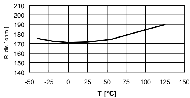
Figure 26. Discharge_RMOS vs temperature
