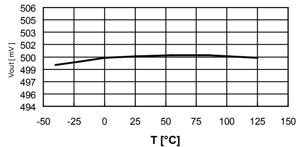
Figure 9. V_{OUT} vs. temperature ( V_{BIAS}@3 V , V_{IN}@V_{OUT} + 0.3 V@1 A )
