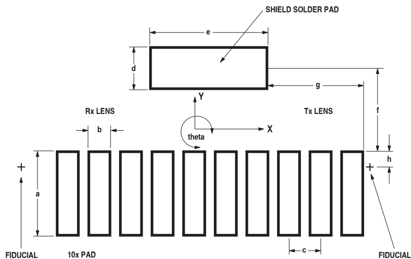
Figure 2. Top view of land pattern.
