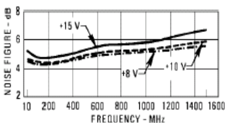
Noise Figure
