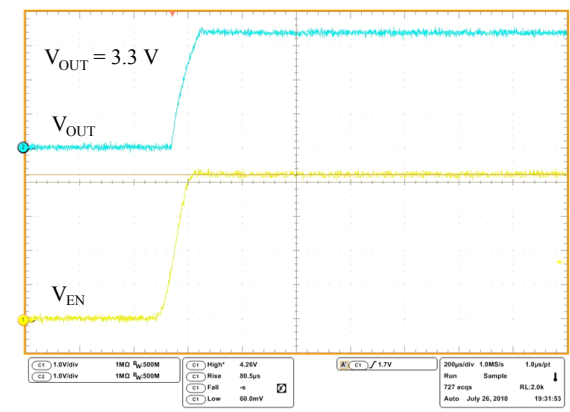
Figure 21. Enable transient
