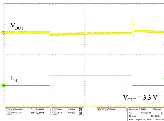
Figure 18. Load transient ( V_{OUT} = 3.3 \text{ V} )
