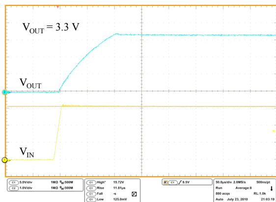
Figure 20. Startup transient
