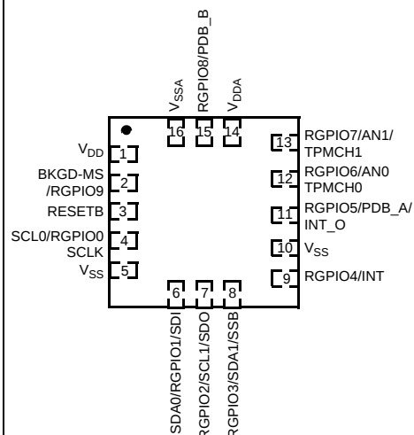
Pin connections
