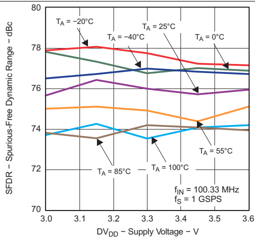
Figure 20. SFDR vs DVDD3 Across Temperature
