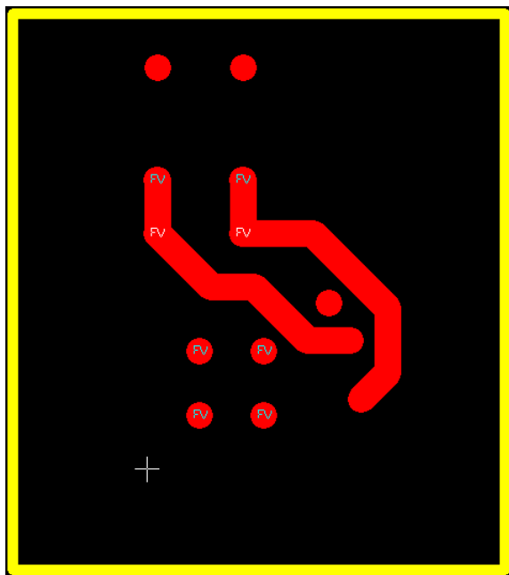
Bottom Copper
