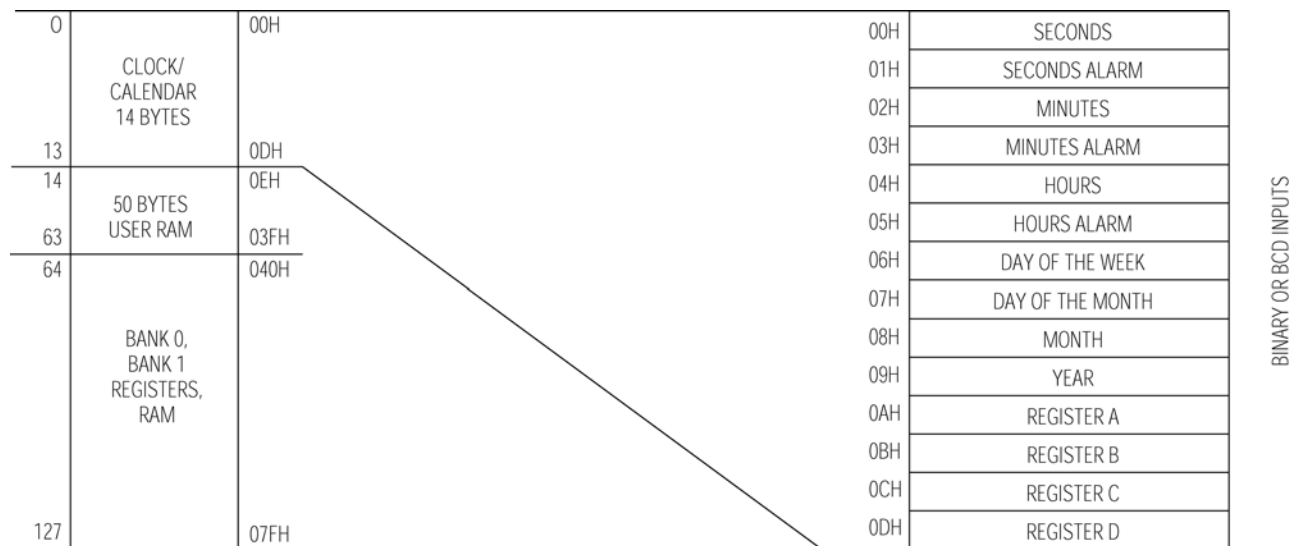
Figure 2. DS1785 REAL-TIME CLOCK ADDRESS MAP
