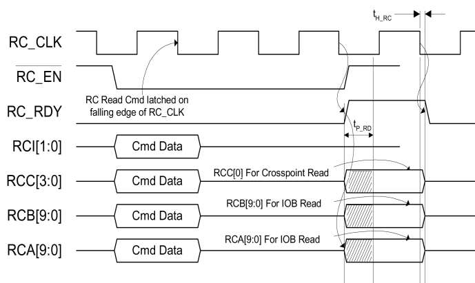
FIGURE 15. RapidConfigure I/O Buffer or Crosspoint Read and Write Cycles
