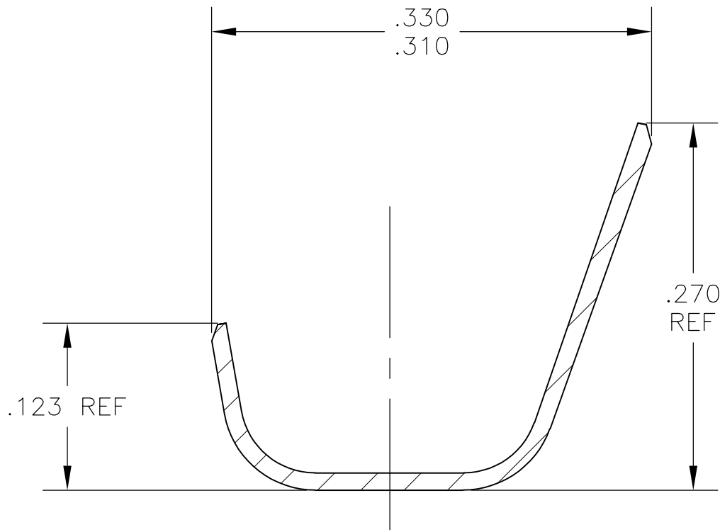
SECTION C-C
