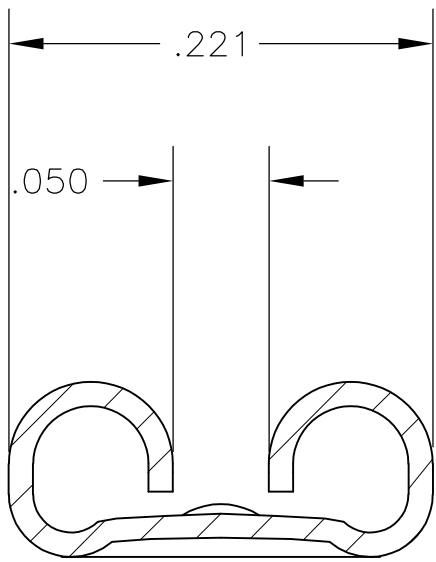
SECTION Y-Y
