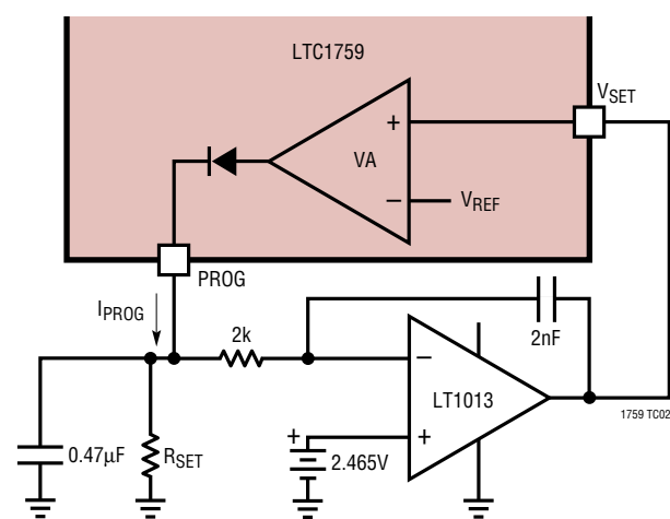
Test Circuit 2
