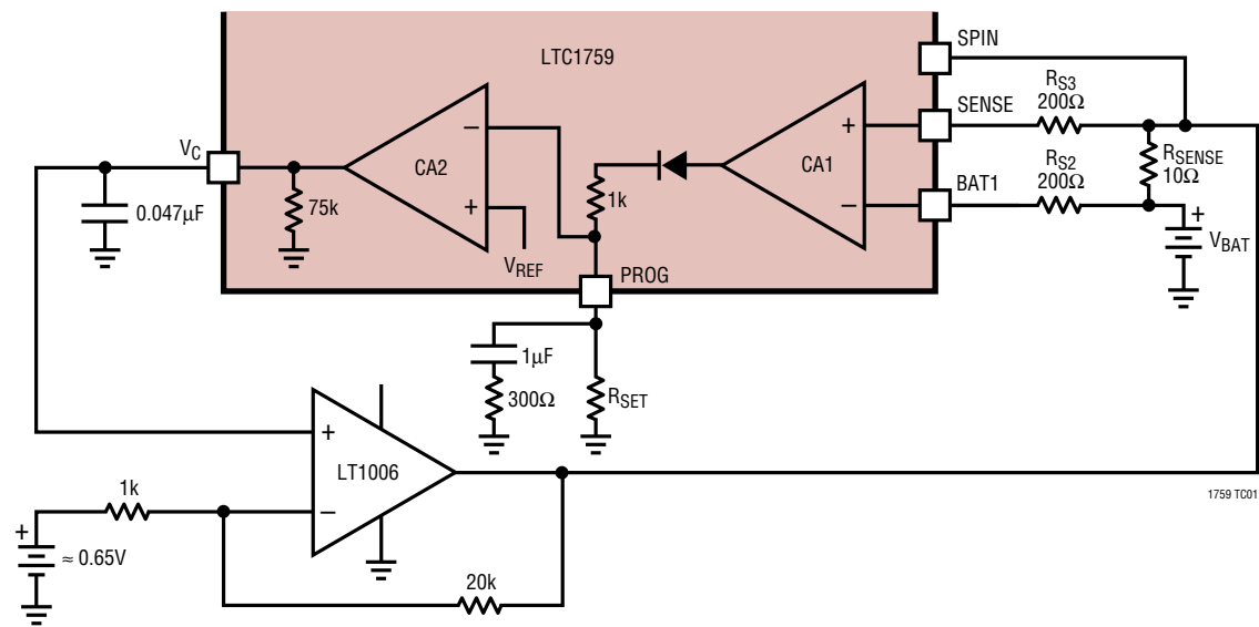
Test Circuit 1
