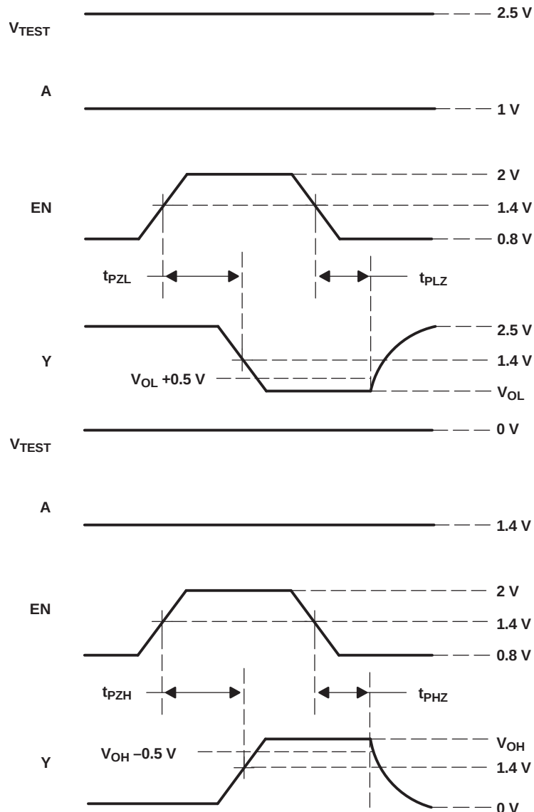
Figure 11. Enable and Disable Time Test Circuit and Waveforms
