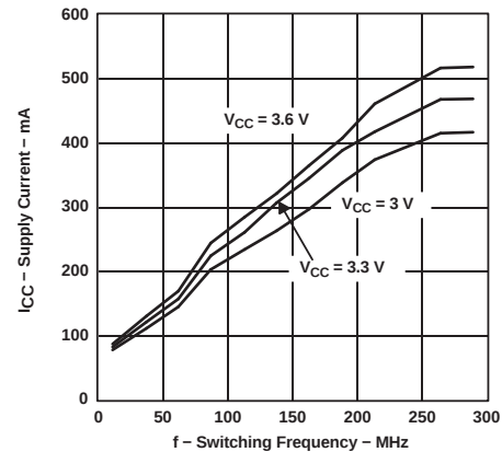
Figure 4. LVDS386 Supply Current vs Switching Frequency
