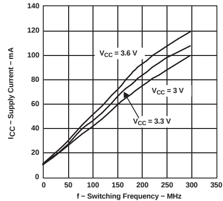
Figure 2. LVDS390 Supply Current vs Switching Frequency
