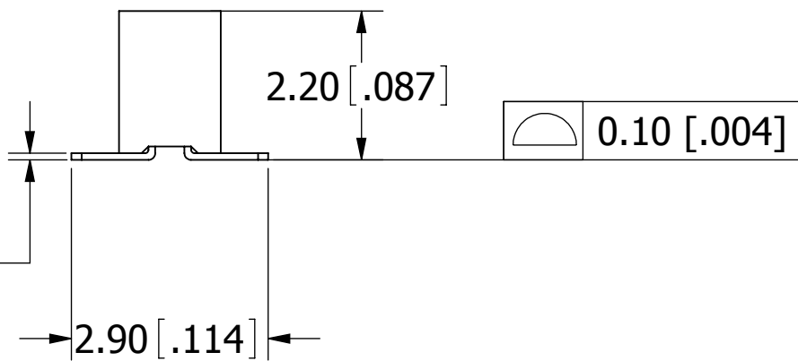
RECOMMENDED PCB LAYOUT SFM210-LP_E-S__-SD-BK
