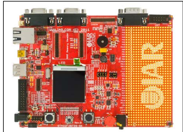
Figure 2. Starter kit
