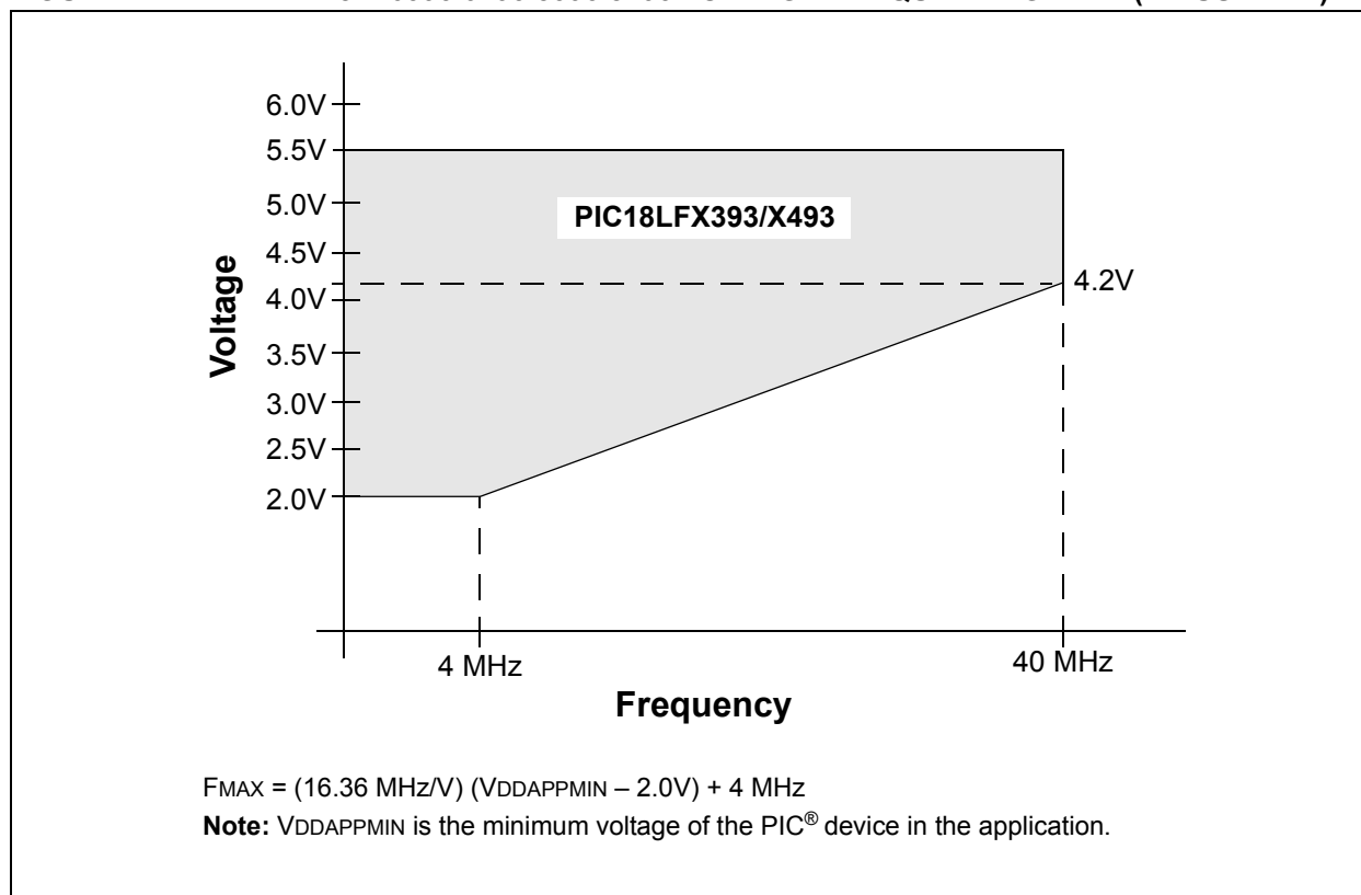
FIGURE 4-2: PIC18LF6393/6493/8393/8493 VOLTAGE-FREQUENCY GRAPH (INDUSTRIAL)
