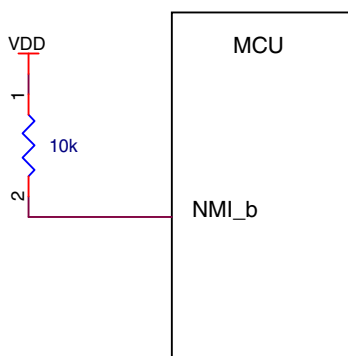
Figure 22. NMI pin biasing
