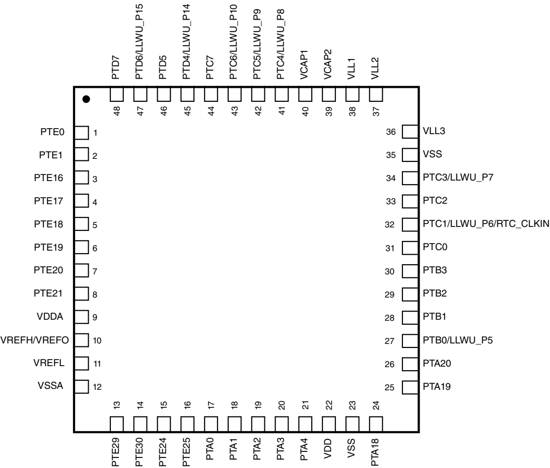
Figure 31. 48 QFN Pinout diagram
