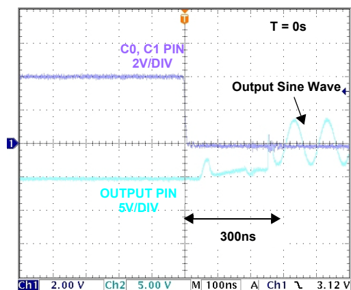
FIGURE 29. POWER ON
