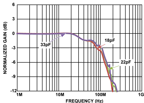
FIGURE 16. SMALL SIGNAL FREQUENCY RESPONSE vs C_{LOAD}
