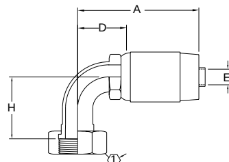
ORS® Swivel 90° elbow (long) FJ9903
