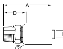
SAE straight thread O-Ring male** FC5809
