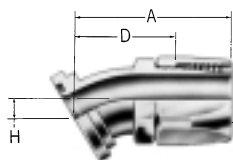
Code 61 SAE J518 30° split flange 190846-
