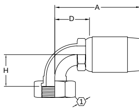
ORS® Swivel 90° elbow (short) FJ9902
