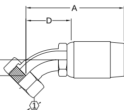
ORS® Swivel 45° elbow FJ9901
