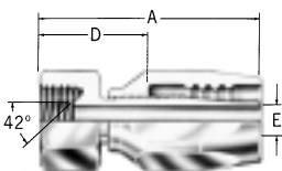
Female inverted flare 403-
