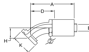
45° elbow split flange FJ9575/FC9724/FJ9767 Code 61 FC9855/FJ9768 Code 62
