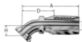
Code 61 SAE J518 45° split flange FC5138-
