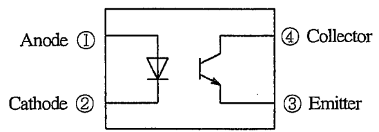
Pin Nos. and internal connection diagram
