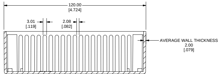
SECTION B-B
