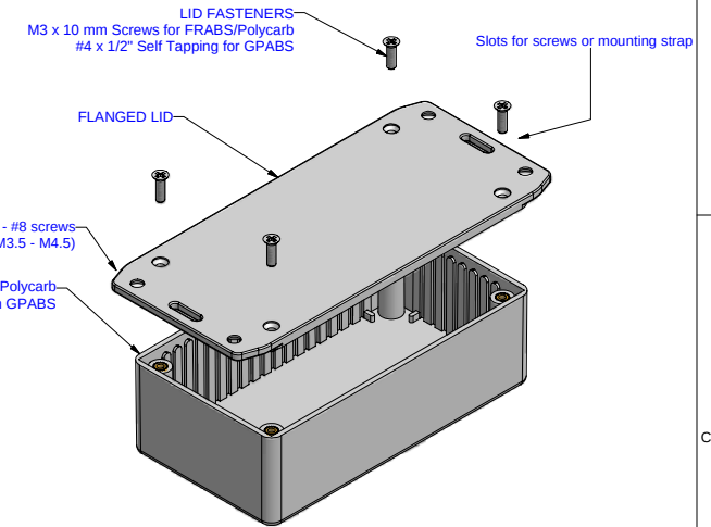
EXPLODED VIEW OF FLANGED ENCLOSURE
