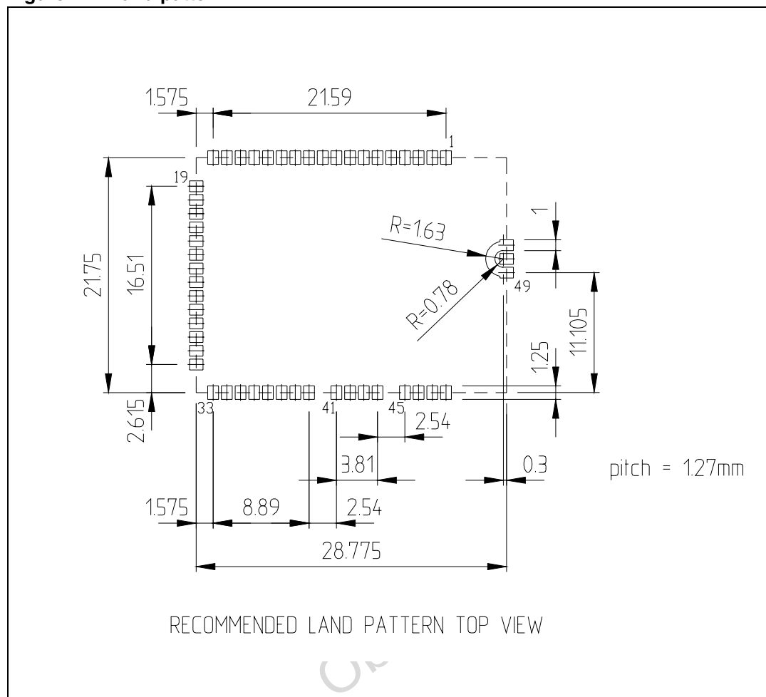
Figure 11. Land pattern
