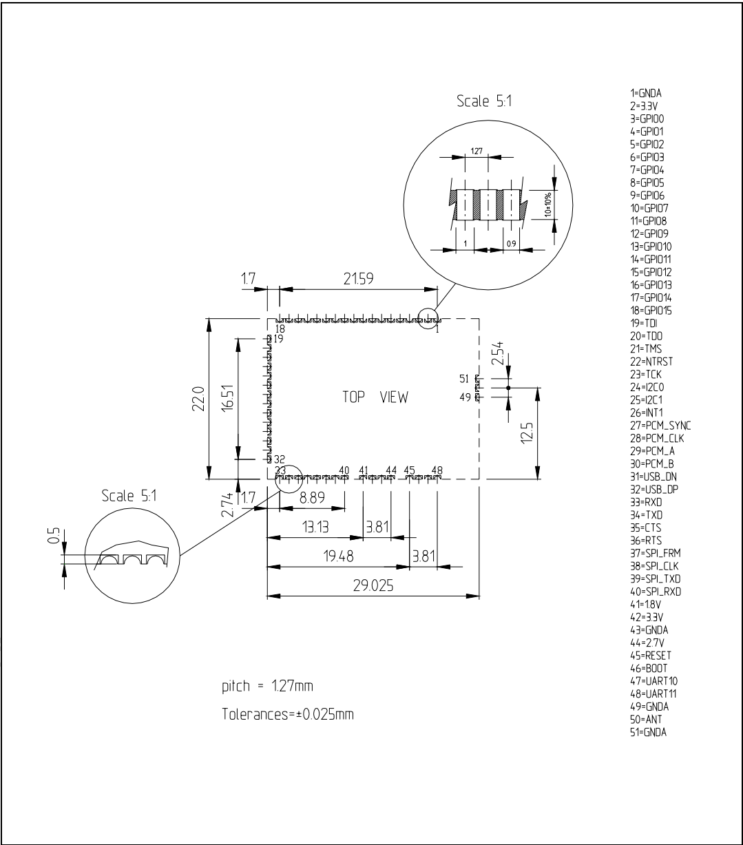
Figure 10. Mechanical dimensions
