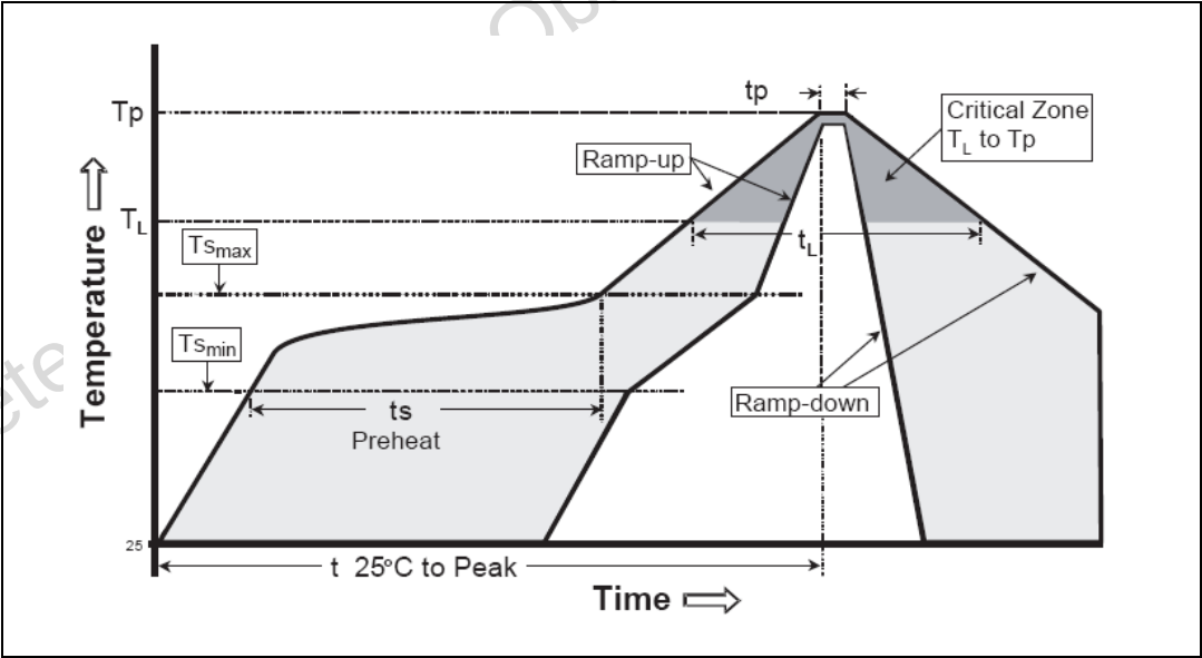
Figure 9. Soldering
